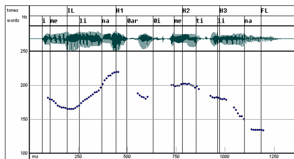
Figure 1: Waveform and pitch contour of the three-word short sentence as realized by GRF2; in the “words” tier, vertical lines correspond to syllable boundaries; in the “tones” tier, they correspond to F0 measurements.
