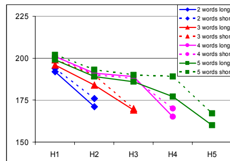
Figure 2: Mean scaling of the five peaks as a function of SENTENCE LENGTH and NO OF WORDS.
