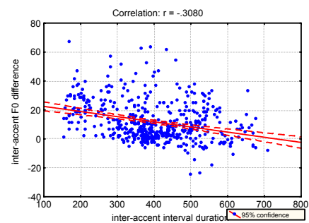
Figure 4: Difference in scaling between successive peaks as a function of inter-accent interval duration; pooled data.
