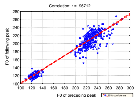
Figure 5: Peak height as a function of the height of the preceding peak.
